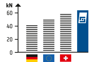
Specified impact load (kN) in comparison: The GOLDBECK solution outperforms the specified standard values for Germany, Europe and Switzerland.
